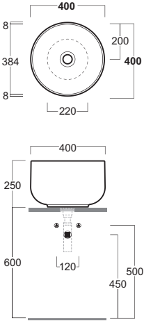
BA 02 Lavabo tondo alto d'appoggio Round countertop washbasin with high rim Ø40.h25
