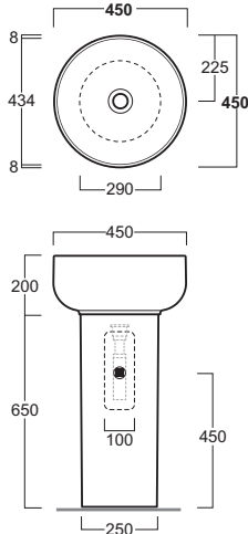
CN 300 Colonna rotonda per BA 01 Rounded pedestal for BA 01 27,5.h65
