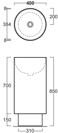
PO 08 Lavabo cilindrico free-standing per installazione centro stanza Cylindric free-standing washbasin for center room installation Ø40.h85
