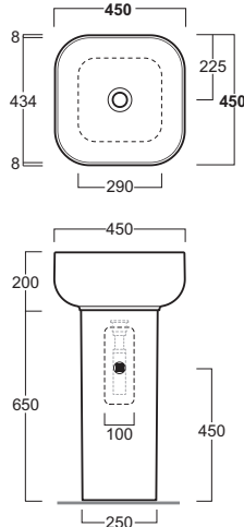
CN 400 Colonna quadrata per BA 03 Squared pedestal for BA 03 27,5.h65
